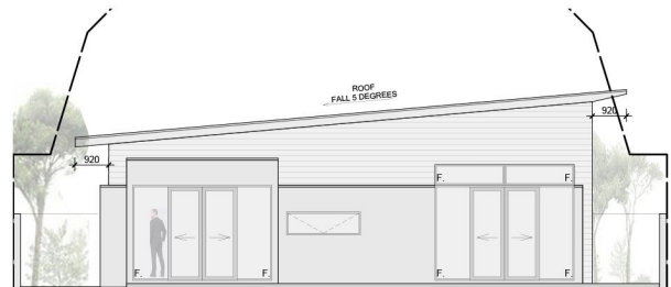
EAST ELEVATION
