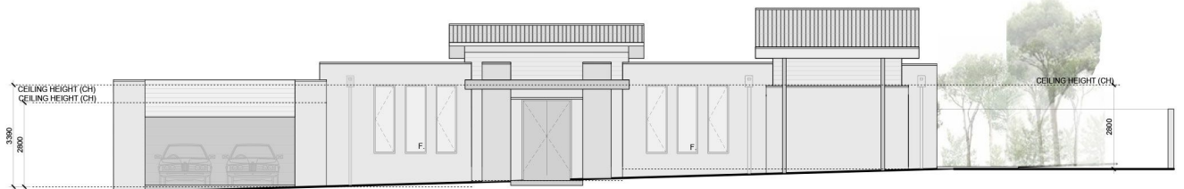
SOUTH ELEVATION
