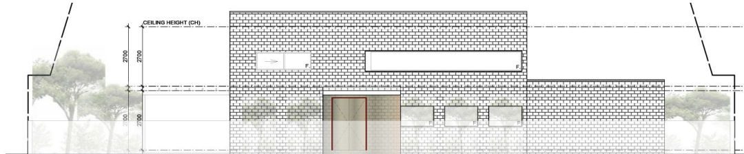
SOUTH ELEVATION
