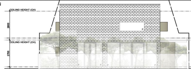
WEST ELEVATION
