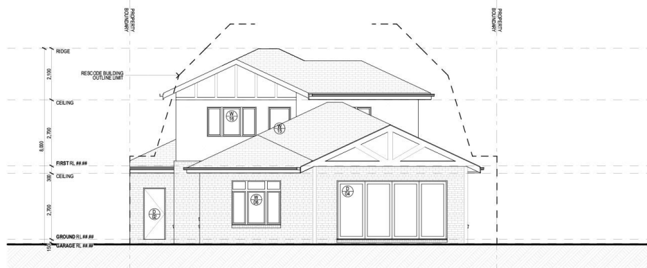
03 REAR ELEVATION 1:100
