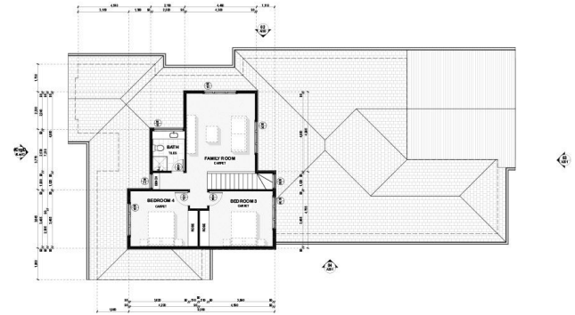
02 FIRST FLOOR PLAN 1:100
