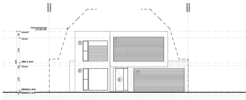
01 FRONT ELEVATION 1:100
