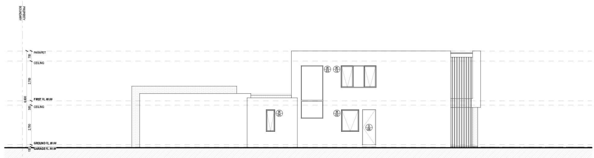
02 SIDE ELEVATION 1:100
